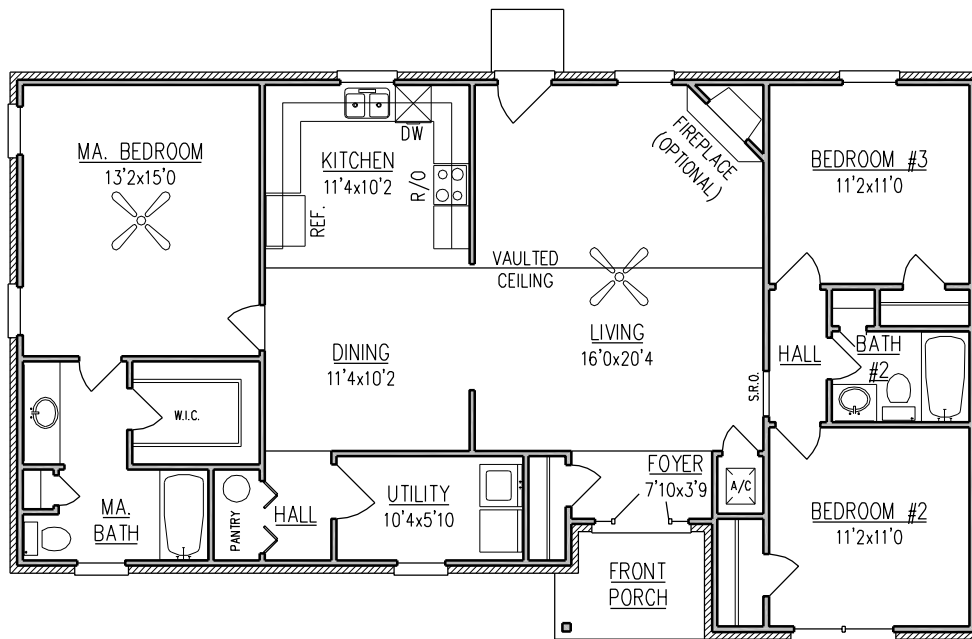
FLOOR PLAN
